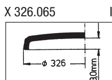
X 326.065 | Laco Mechanic
