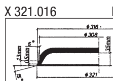
X 321.016 | X 322.022
