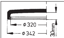
Omega Speedmaster 5077
