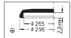
Citizen 54-05921 S
